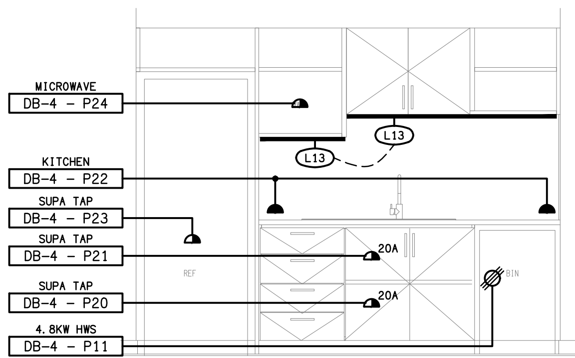
DETAIL A STAFF ROOM KITCHENETTE SCALE 1: 25
